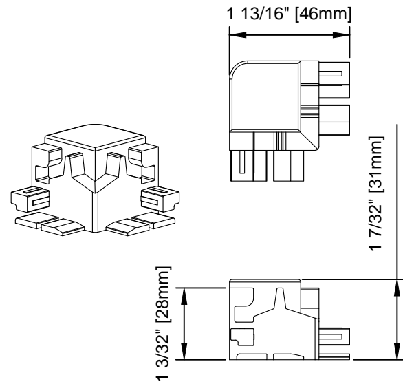
INTERIOR CORNER CONNECTOR
