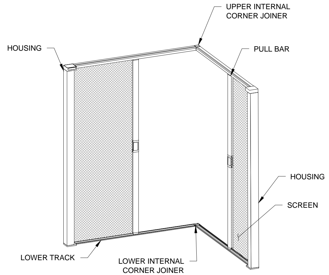
INTERNAL CORNER 3D VIEW
