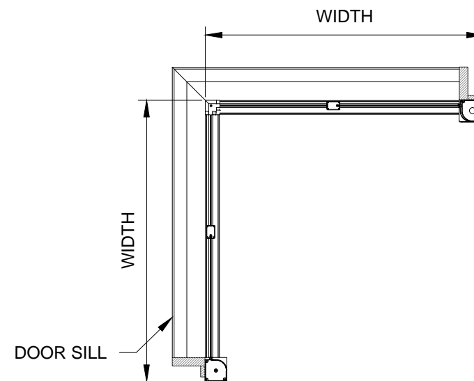
INTERNAL CORNER SECTION VIEW
