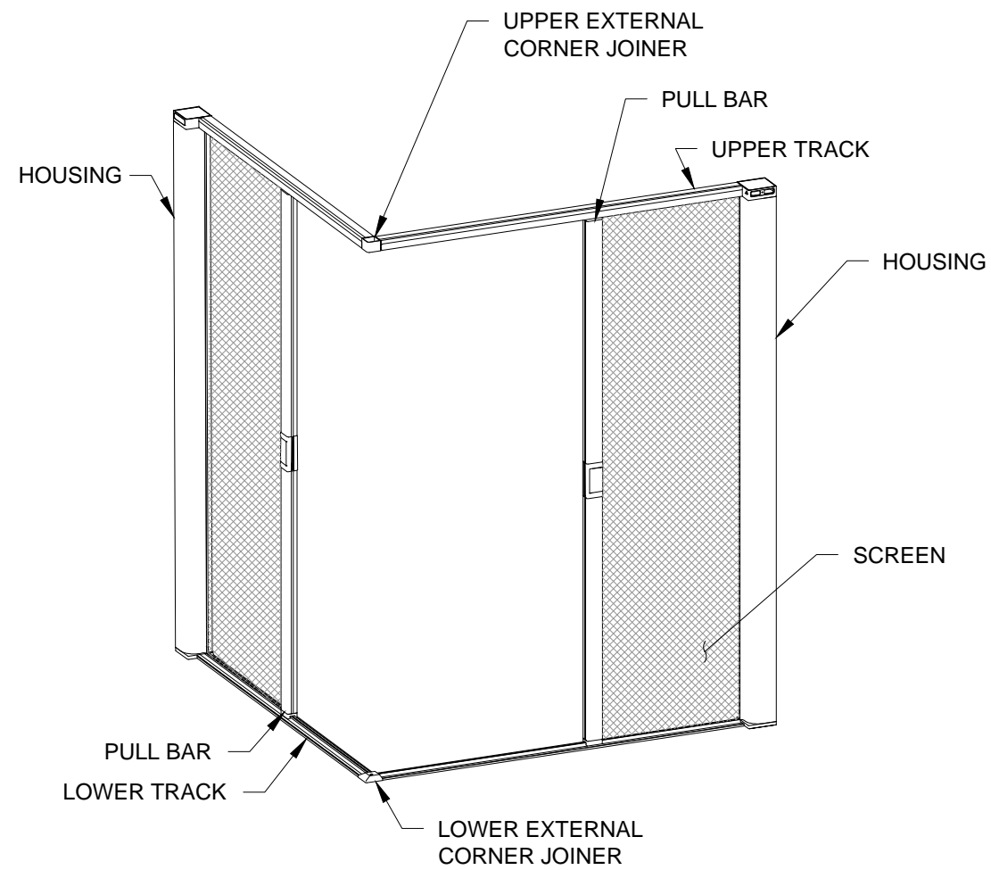
EXTERNAL CORNER 3D VIEW
