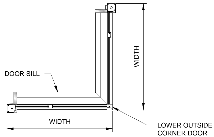
EXTERNAL CORNER SECTION VIEW
