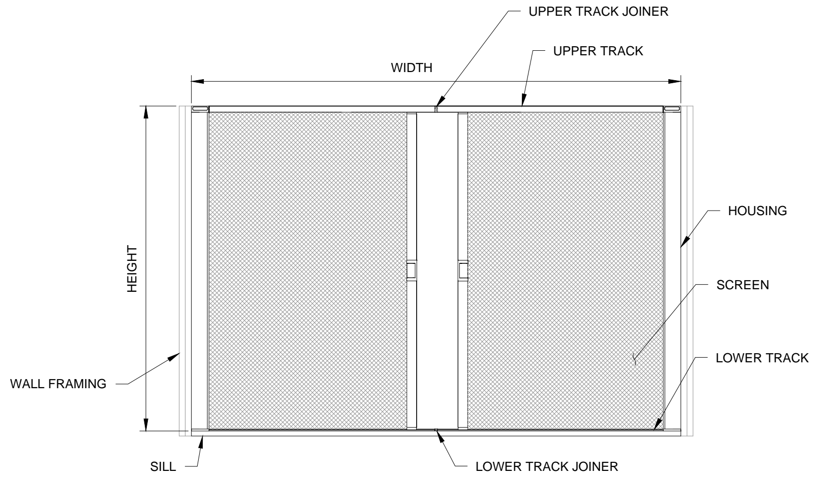
FRONT ELEVATION
