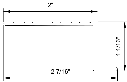
INTERIOR SILL ADAPTER (VS-40114)
