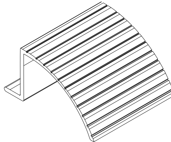
OVER SILL ADAPTER (VS-40116)
